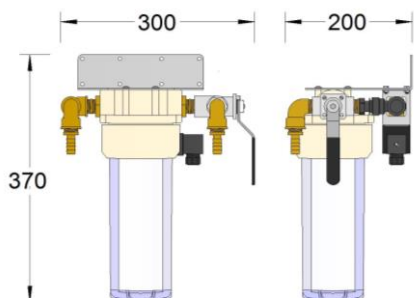
Pre-filter Assembly
