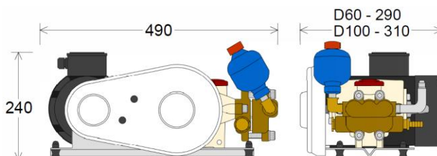
High Pressure Pump Assembly
